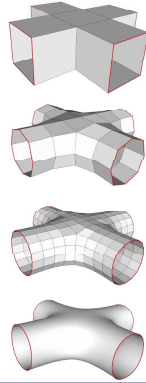
(Catmull-Clark in action)
